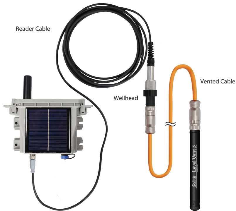
Figure 2-3 LevelVent Connection
