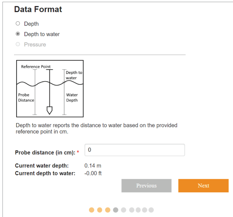
Figure 4-5 SolSat 5 Depth to Water Measurement
